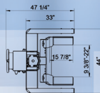
Adjustable forks
