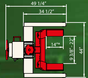
Adjustable fork
