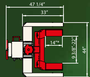
Adjustable fork
